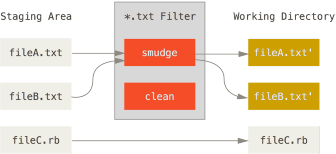
Figure 144. “smudge” 过滤器会在文件被检出时触发
